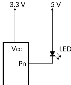
Figure 18. Device Supplied by Lower Voltage
