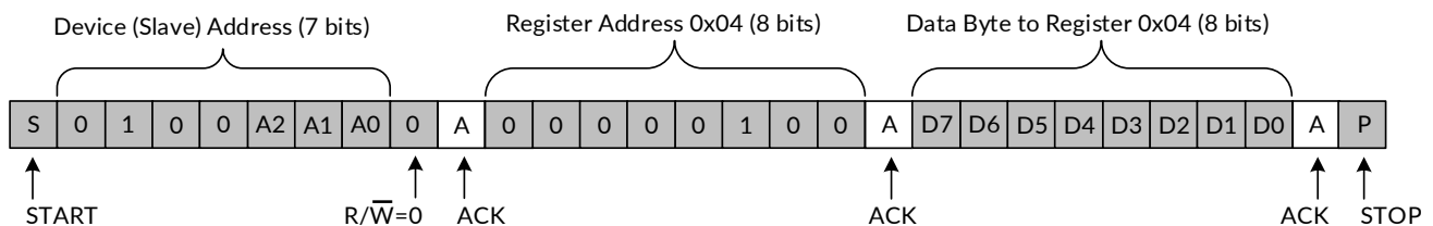
Figure 9. Write to the Polarity Inversion Register
