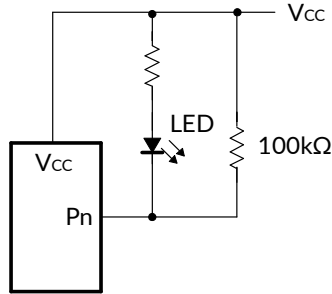
Figure 17. High-Value Resistor in Parallel With LED
