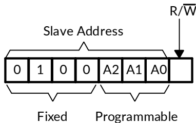
Figure 14. RS29555 Address
