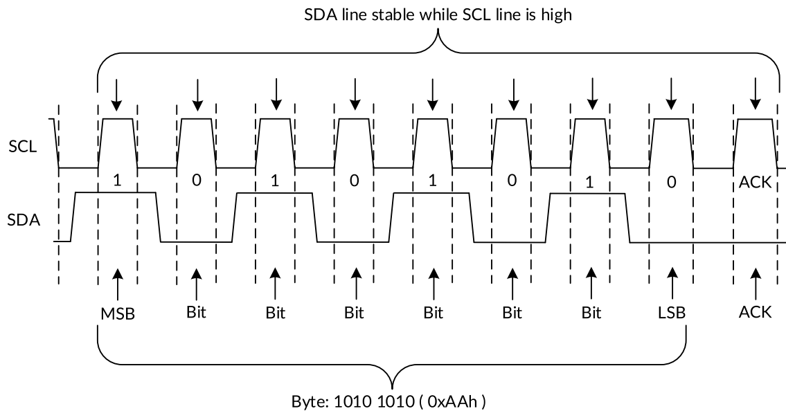
Figure 7. Bit Transfer
