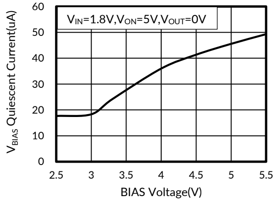
Figure 3. V_{\text{BIAS}} Quiescent Current vs BIAS Voltage
