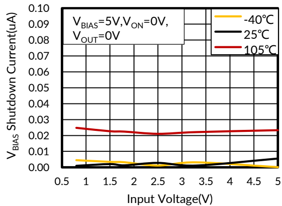
Figure 6. V_{\text{BIAS}} Shutdown Current vs Input Voltage
