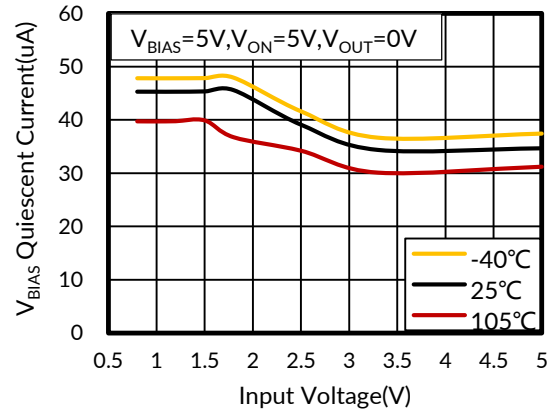
Figure 4. V_{\text{BIAS}} Quiescent Current vs Input Voltage
