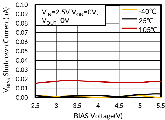
Figure 5. V_{\text{BIAS}} Shutdown Current vs BIAS Voltage
