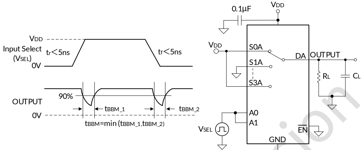
Figure 15. Break-Before-Make Delay Measurement Setup
