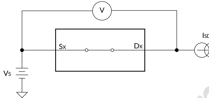
Figure 11. On-Resistance Measurement Setup
