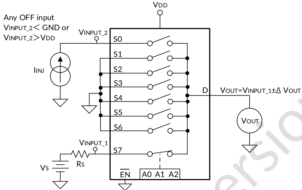
Figure 21. Injection Current Measurement Setup
