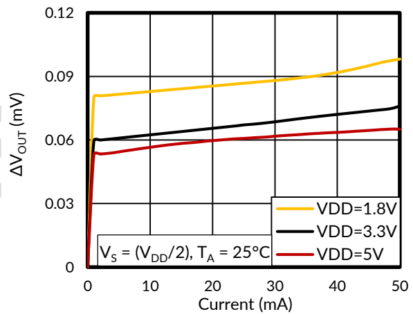
Figure 10. Injection Current vs Maximum Output Voltage Shift
