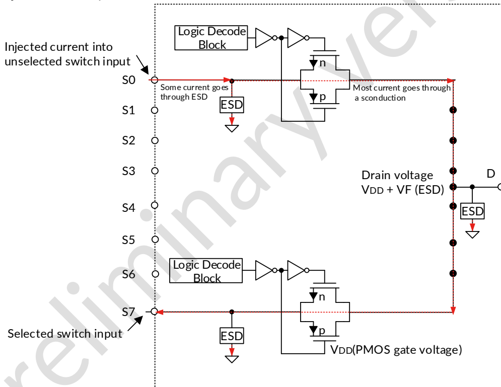
Figure 22. Simplified Diagram of Typical CMOS Switch and Associated Injected Current Path
