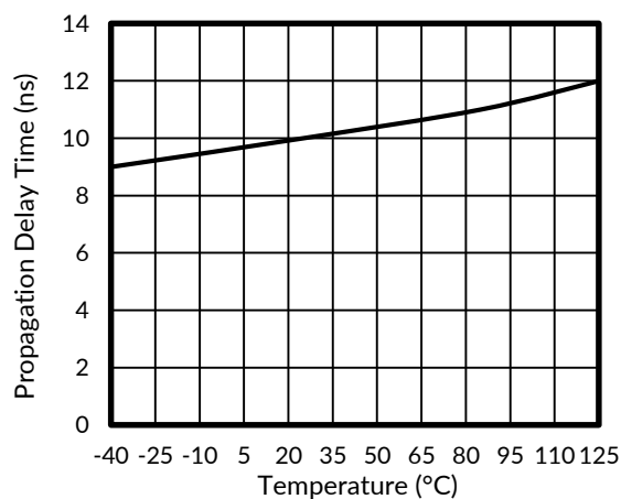
Figure 2. T_{PD} vs Temperature
