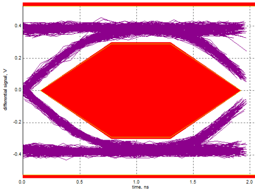
Figure 15. Eye Pattern: 480-Mbps USB Signal with HSD1 Path
