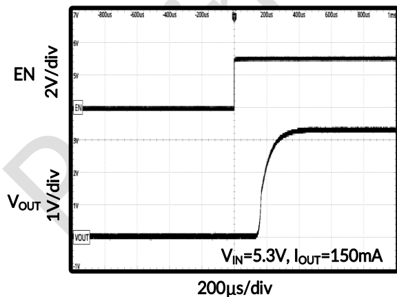
Figure 23. Turn On
