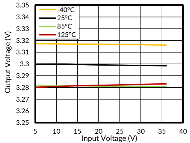
Figure 8. Line Regulation
