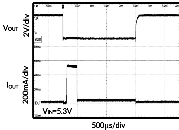
Figure 25. Turn On First, Then Short Circuit
