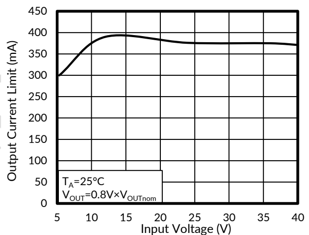
Figure 16. Output Current Limit vs Input Voltage
