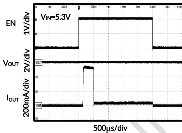
Figure 27. Short Circuit First, Then Enable
