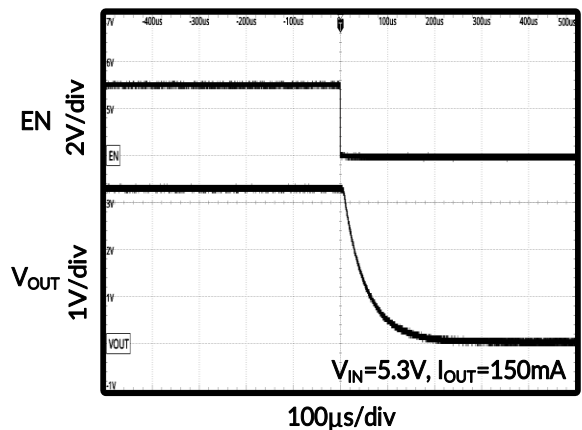
Figure 24. Turn Off
