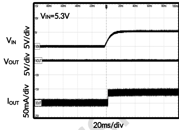
Figure 26. Short Circuit First, Then VIN Power ON
