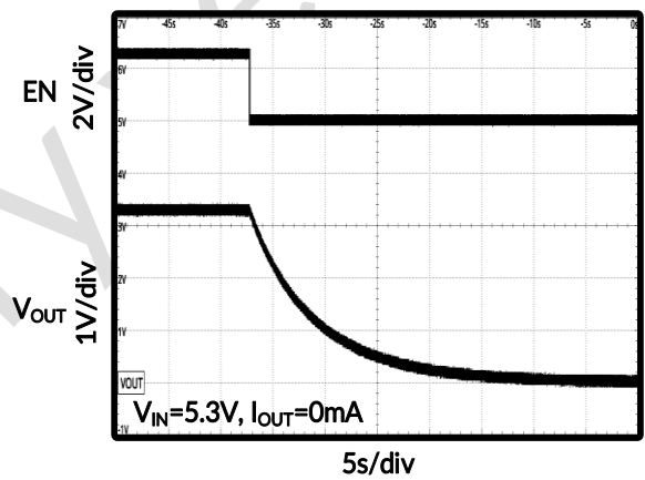
Figure 22. Turn Off
