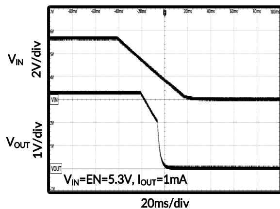
Figure 18. Power Off
