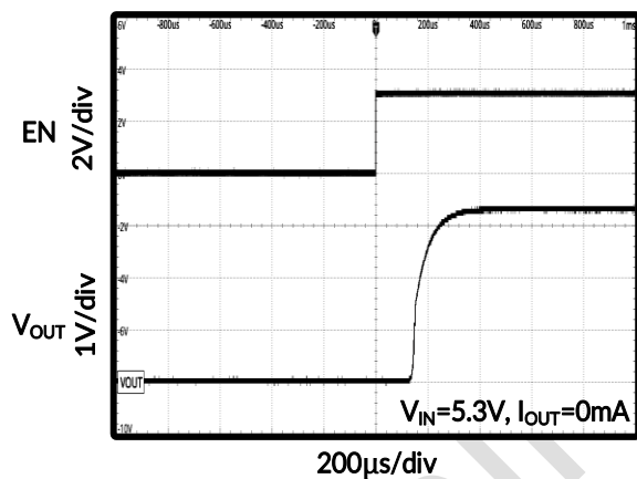
Figure 21. Turn On
