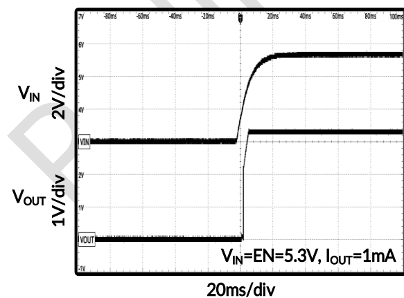
Figure 17. Power On
