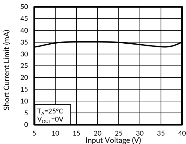
Figure 15. Short Current Limit vs Input Voltage
