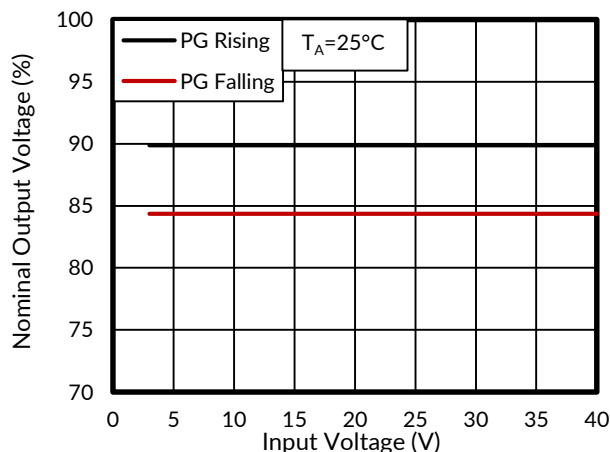
Figure 17. Power-Good Threshold Voltage vs Input Voltage
