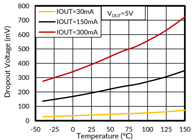
Figure 12. Dropout Voltage vs Junction Temperature
