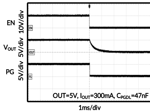
Figure 36. Start-Up Through EN
