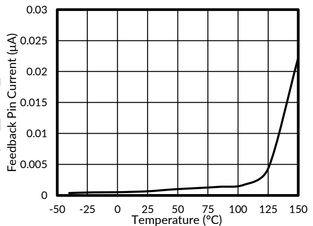
Figure 10. Feedback Pin Current vs Junction Temperature
