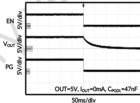
Figure 34. Start-Up Through EN
