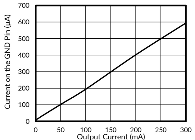
Figure 6. Ground Pin Current vs Output Current
