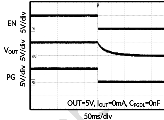
Figure 38. Start-Up Through EN
