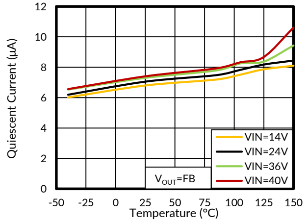
Figure 2. Quiescent Current vs Junction Temperature
