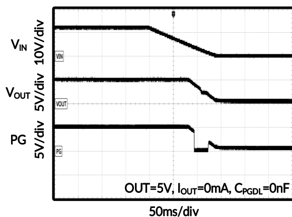
Figure 30. Start-Up Through V_{IN}
