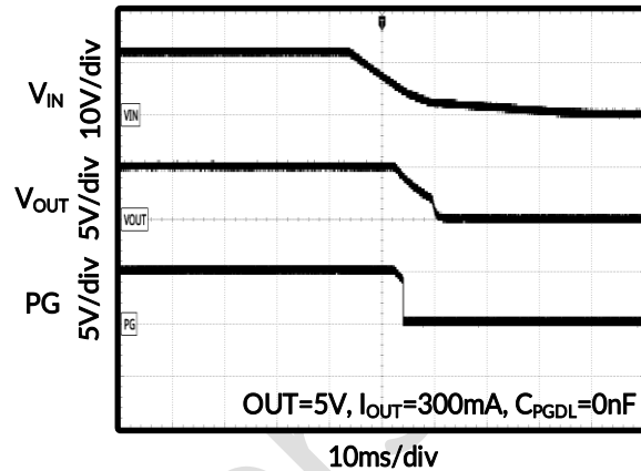
Figure 32. Start-Up Through V_{IN}
