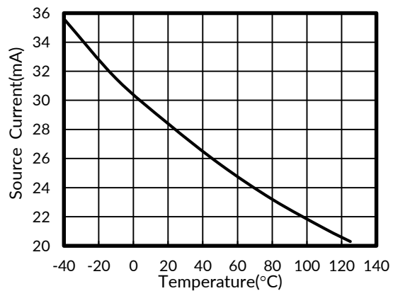
Figure 6. Source Current vs Temperature
