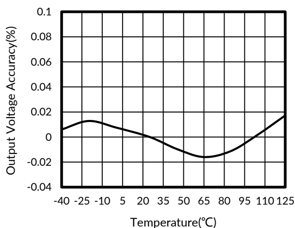
Figure 4. Output Voltage Accuracy vs Temperature
