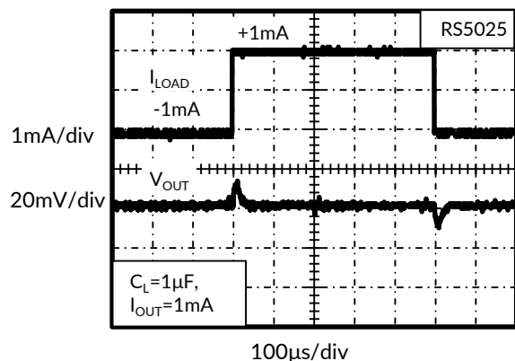
Figure 13. Load Transient
