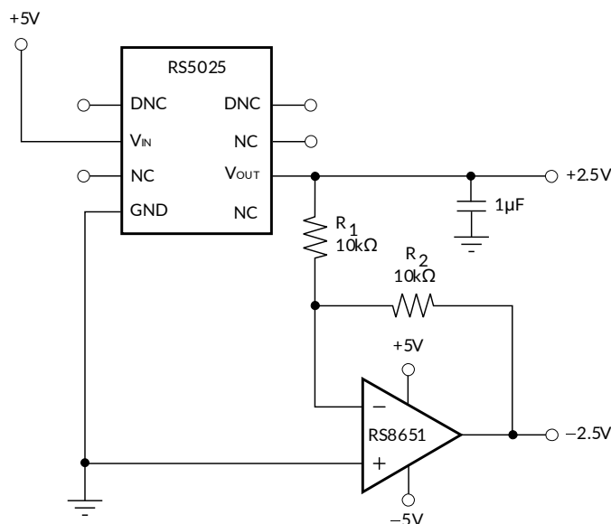
Figure 23. The RS5025 and RS8651 Create Positive and Negative Reference Voltages
