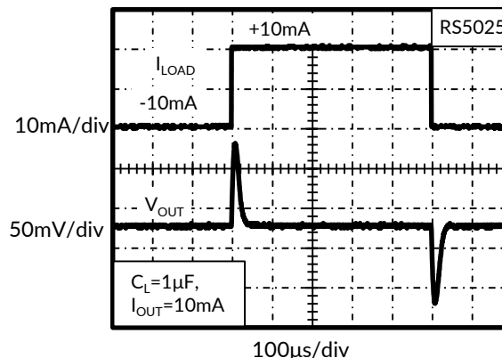
Figure 14. Load Transient
