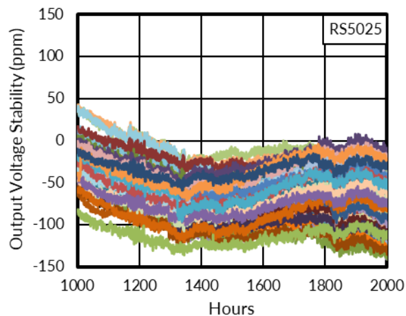
Figure 20. Long - Term Stability (Second 1000 hours)
