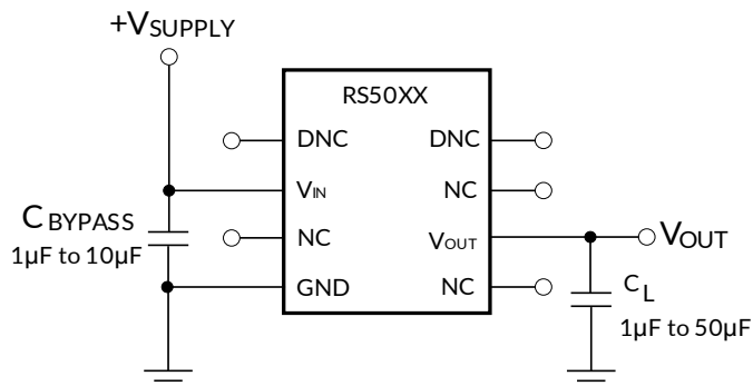
Figure 22. Basic Connections
