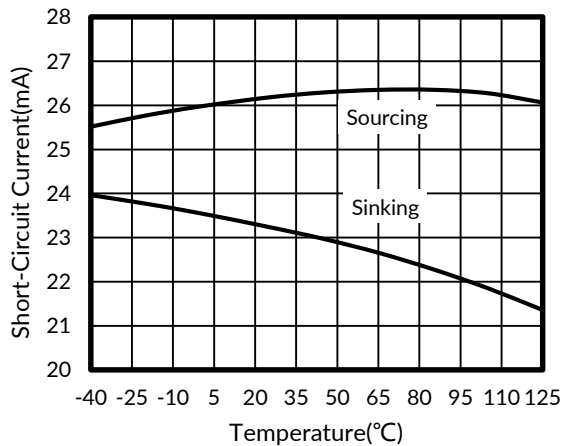
Figure 9. Short Circuit Current vs Temperature
