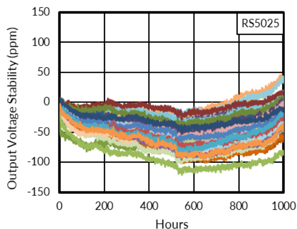
Figure 19. Long - Term Stability (First 1000 hours)
