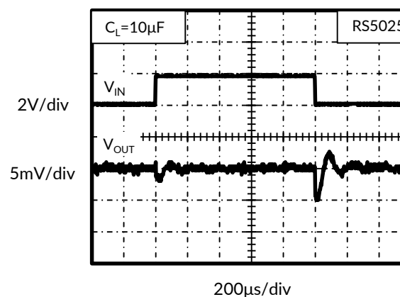
Figure 18. Line Transient
