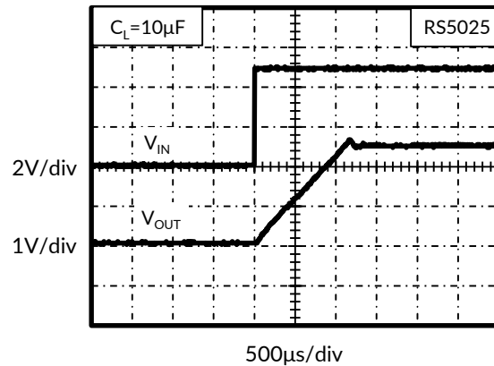
Figure 12. Start-up
