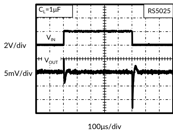
Figure 17. Line Transient
