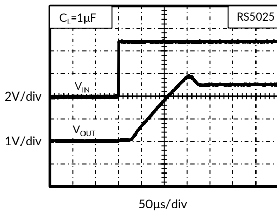
Figure 11. Start-up
