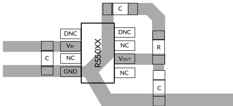
Figure 24. Layout Example
