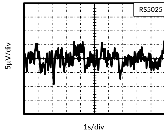
Figure 10. Noise
