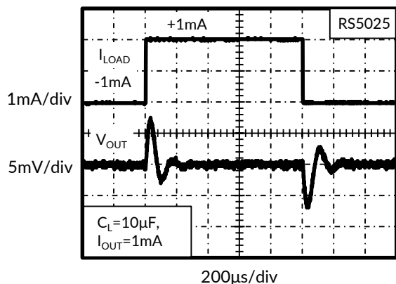
Figure 15. Load Transient
