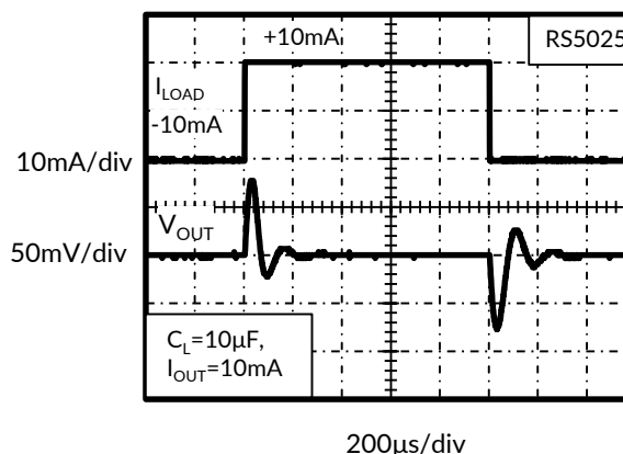
Figure 16. Load Transient
