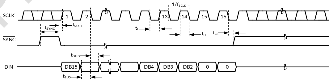
Figure 2. RS1300 Timing
