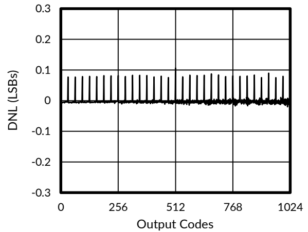
Figure 4. DNL at V_A = 5 \text{ V}
