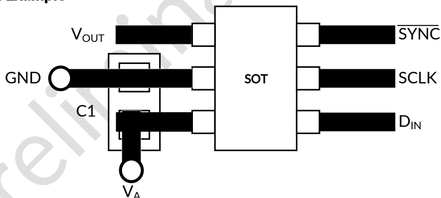
Figure 38. Typical Layout
