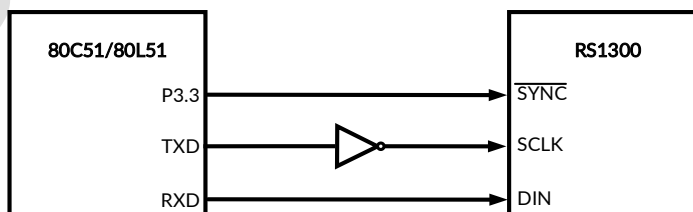
Figure 36. 80C51/80L51 Interface
