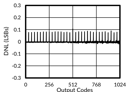
DNL vs Output Code
