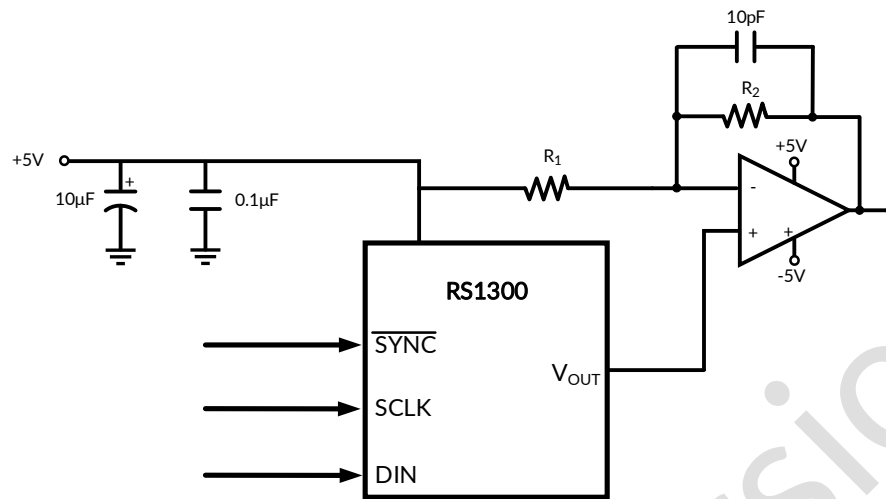
Figure 37. Bipolar Operation
