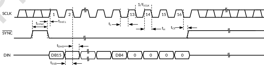
Figure 2. RS1380 Timing
