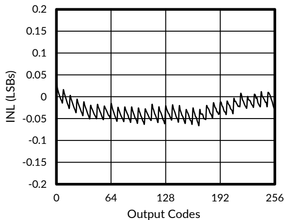
Figure 5. INL at V_A = 3\text{ V}
