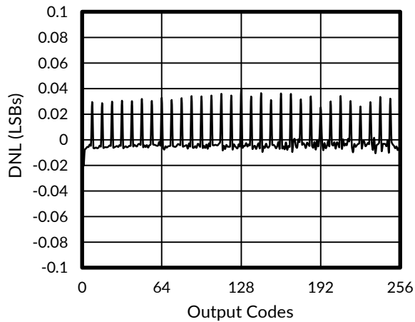
Figure 3. DNL at V_A = 3\text{ V}
