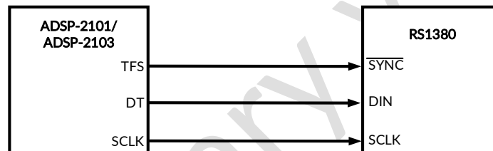
Figure 35. ADSP-2101/2103 Interface
