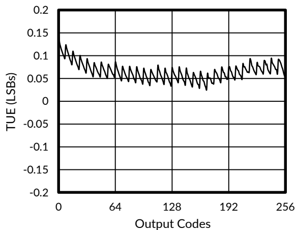
Figure 7. TUE at V_A = 3\text{ V}
