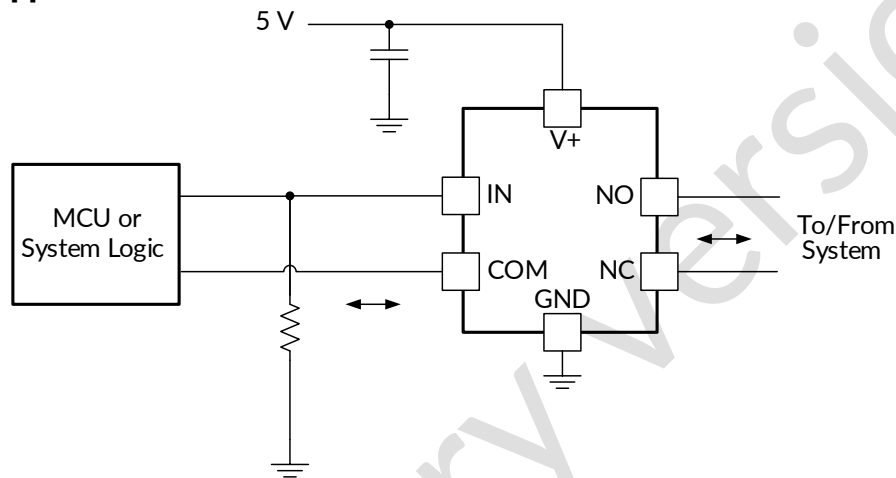
Figure 21. System Schematic for RS2057A-Q1
