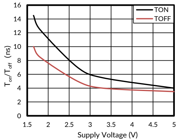
Figure 6. T on and T off vs Supply Voltage
