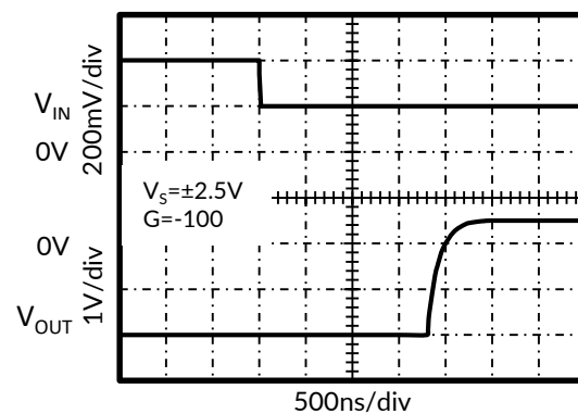
Figure 12. Negative Overvoltage Recovery
