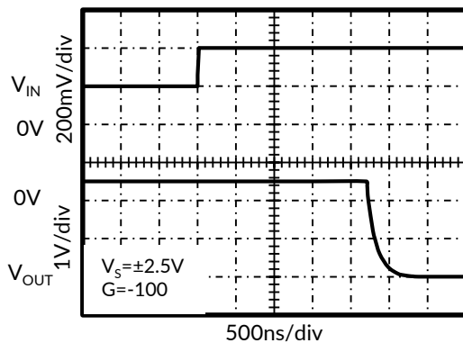
Figure 11. Positive Overvoltage Recovery
