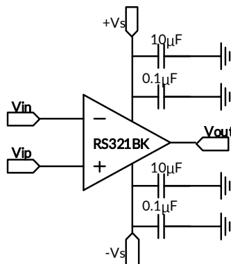
Figure 13. Amplifier with Bypass Capacitors
