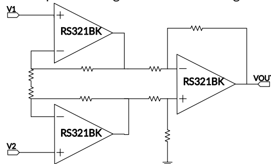
Figure 14. Amplifier Instrumentation Amplifier
