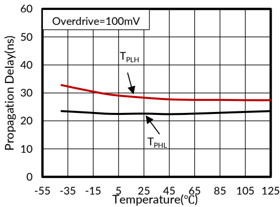
Figure 11. Propagation Delay vs Temperature
