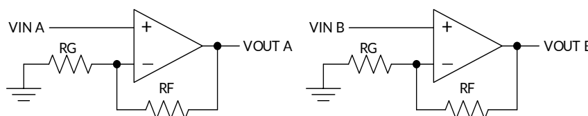
Figure 13. Schematic Representation
