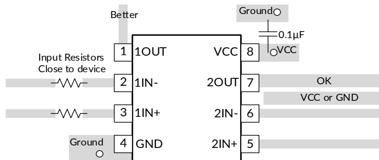
Figure 25. LM2903-Q1 Layout Example
