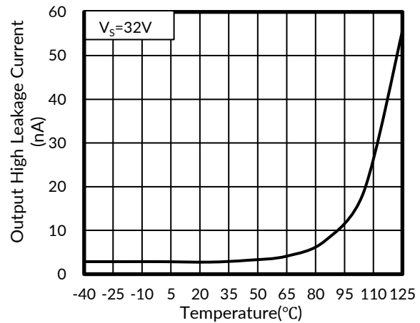
Figure 22. Output High Leakage Current vs Temperature
