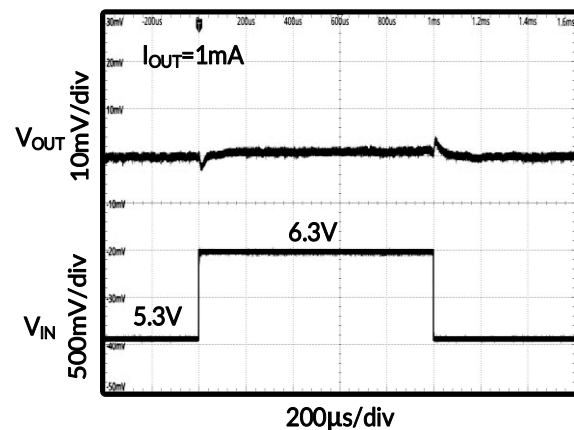
Figure 23. Line Transient Response
