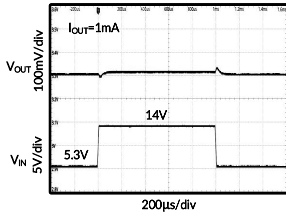
Figure 25. Line Transient Response
