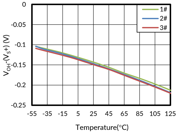
Figure 7. Output Swing from Rail vs Temperature
