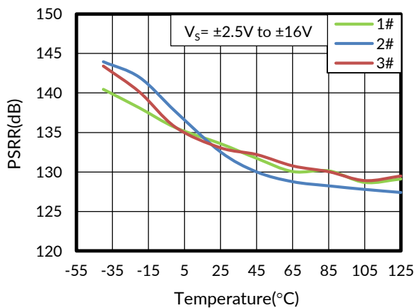
Figure 11. Power-Supply Rejection Ratio vs Temperature
