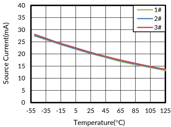
Figure 9. Source Current vs Temperature
