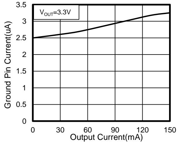
Figure 8. Ground Pin Current vs Load Current
