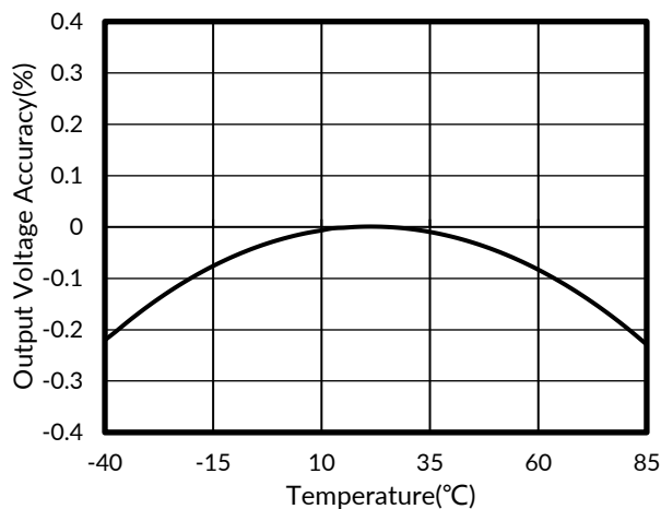
Figure 9. Output Voltage Accuracy vs Temperature
