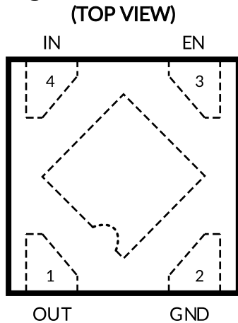
XDFN1X1-4
