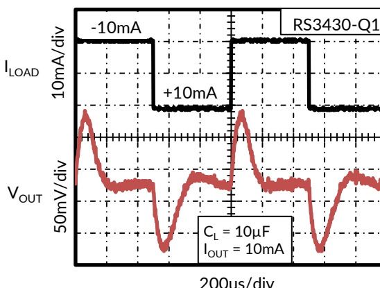
Figure 12. Load Transient
