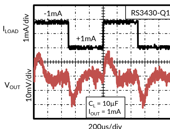
Figure 10. Load Transient
