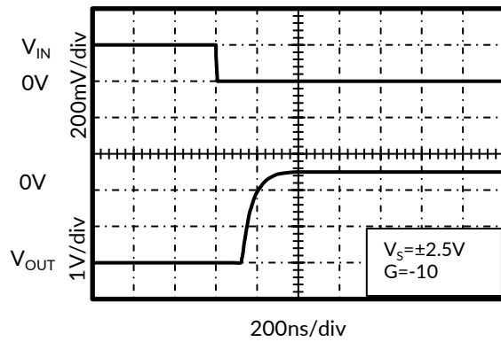
Figure 13. Negative Overload Recovery
