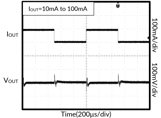
Figure 2. Load-Transient Response
