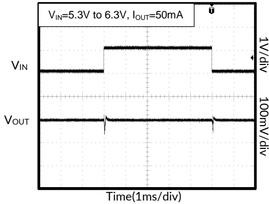
Figure 1. Line-Transient Response
