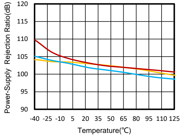
Figure 8. Power-Supply Rejection Ratio vs Temperature
