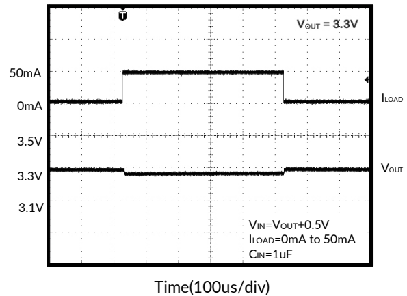
Figure 4. Load-Transient Response
