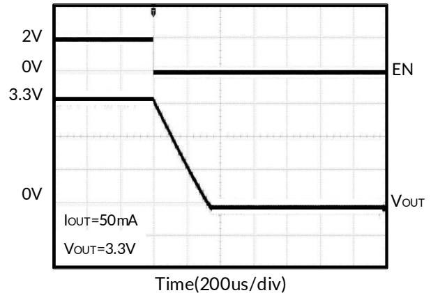
Figure 2. Shutdown
