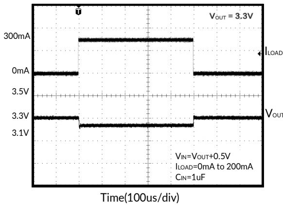
Figure 3. Load-Transient Response
